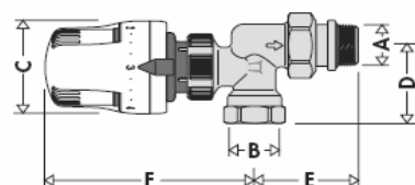
Equerre inverse
